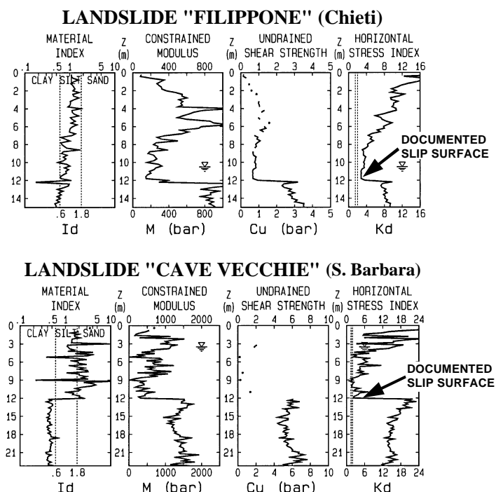
Fig. 40. Examples of K_D \gg 2 in documented slip surfaces in two OC clay slopes - (1 bar = 100 kPa)
