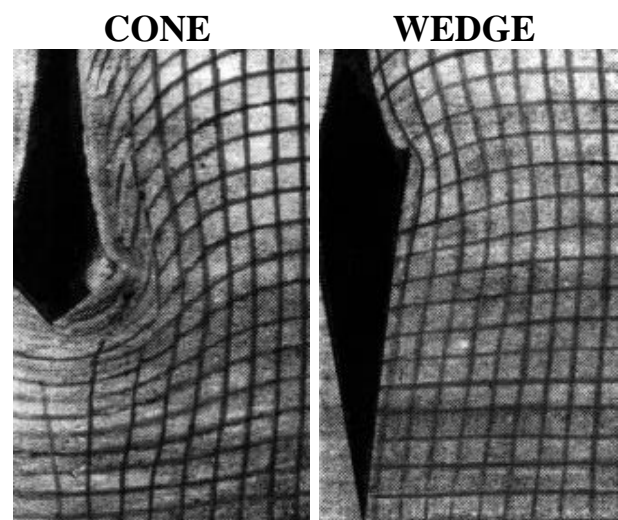
Fig. 46. Deformed grids by Baligh & Scott (1975)
