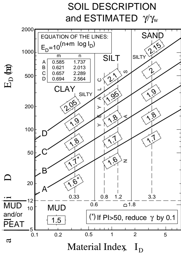
Fig. 16. Chart for estimating soil type and unit weight g (normalized to g_w = g water) - Marchetti & Crapps 1981 - (1 bar = 100 kPa)
