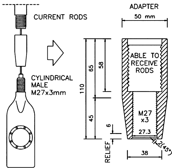
Fig. 8. Lower adaptor connecting the DMT blade to the push rods
