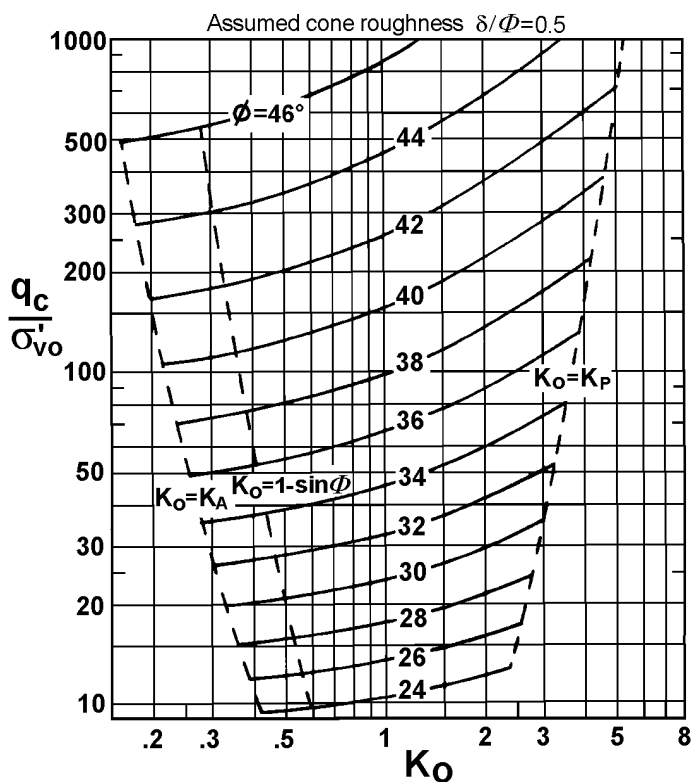
Fig. 24. Chart q_c - K_0 - f – graphical equivalent of the Durgunoglu & Mitchell theory (worked out by Marchetti 1985)
